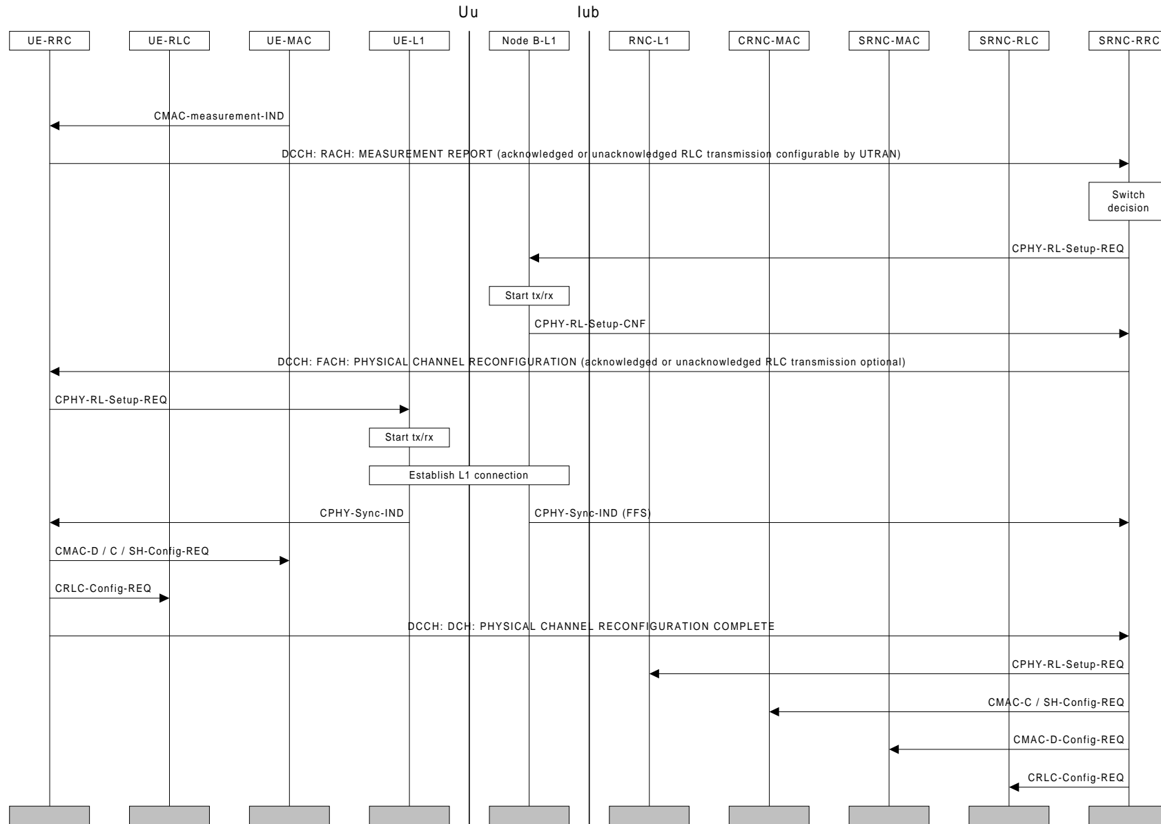
Figure 14: UE-Originated DCH Activation
