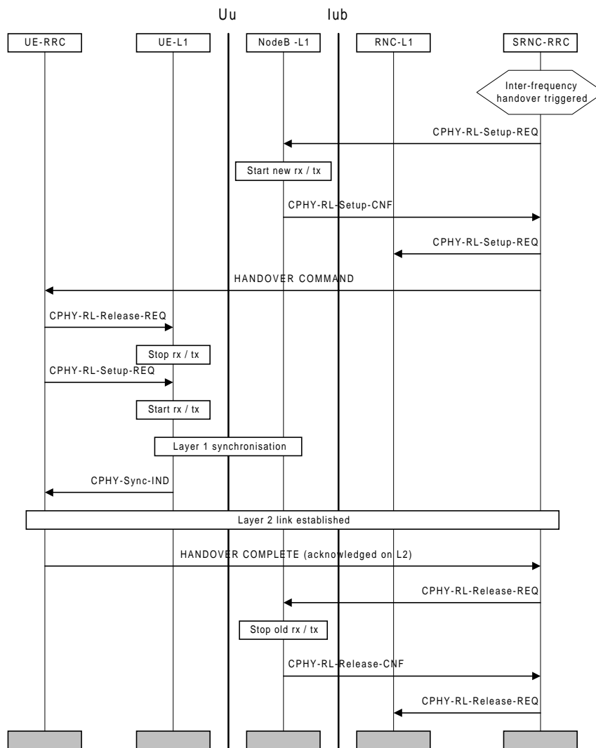
Figure 34: Hard handover
