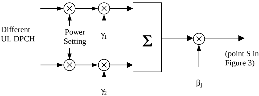
Figure 4: Combination of different physical channels in uplink
