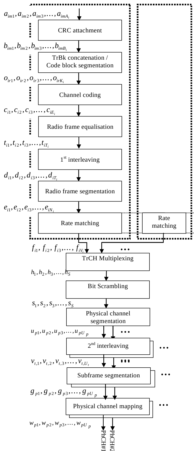
Figure 1A: Transport channel multiplexing structure for uplink and downlink of 1.28Mcps TDD
