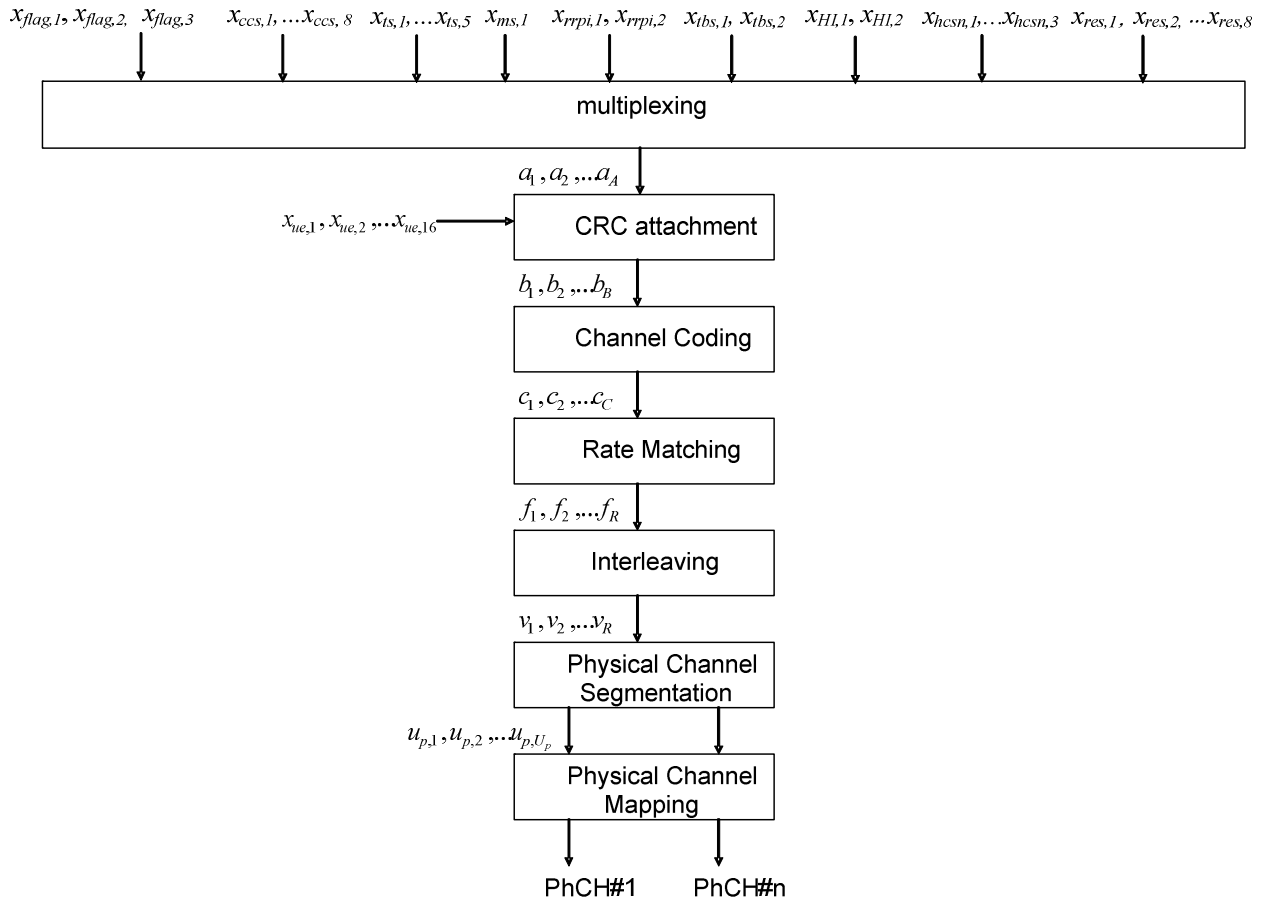
Figure 19E: Coding and Multiplexing for HS-SCCH type 6
