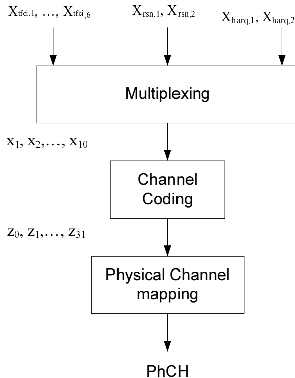
Figure 24A: Coding chain for E-UCCH
