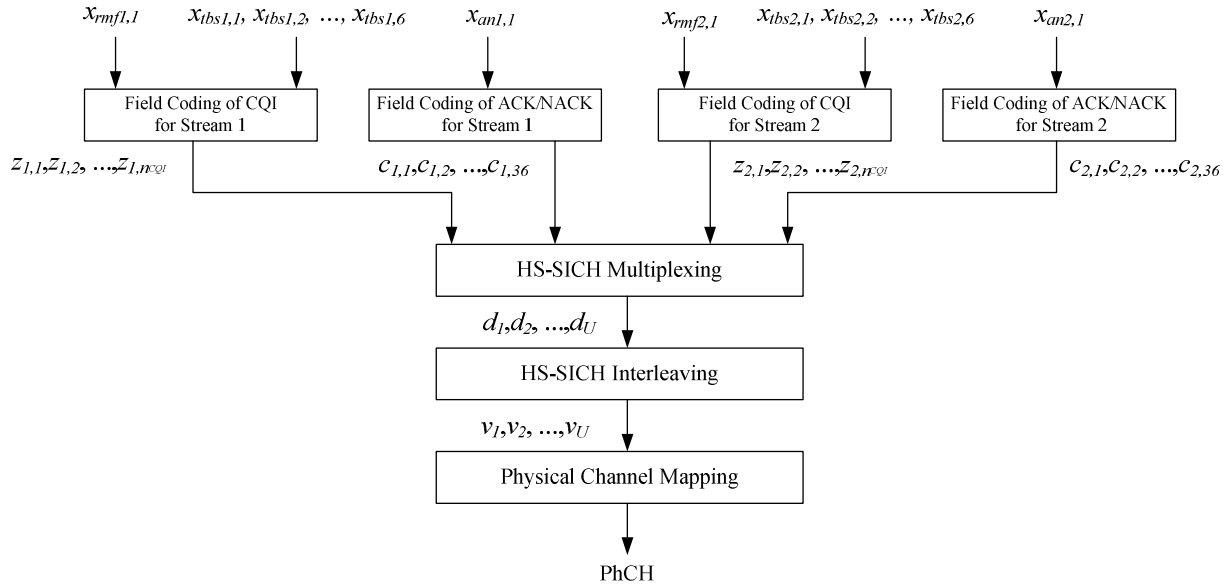
Figure 20A: Coding and multiplexing for HS-SICH type 2
