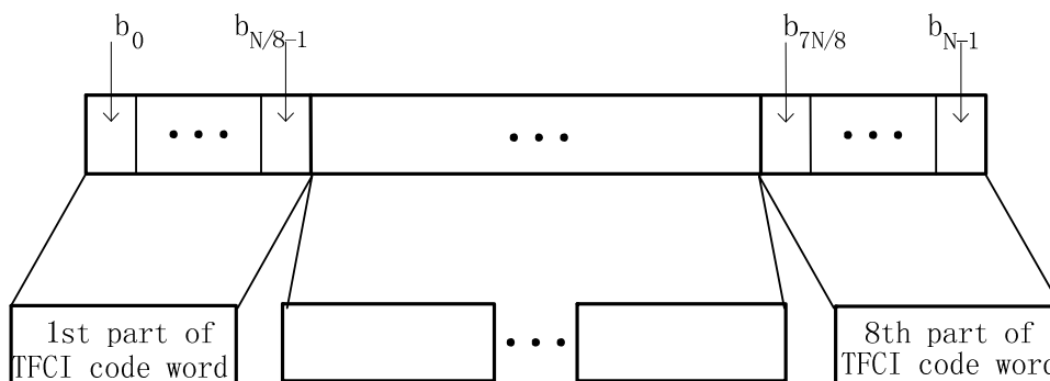
Figure 9A: Mapping of TFCI code word bits to TFCI position in 1.28 Mcps TDD option for downlink MBSFN, where N = N TFCI code word .
