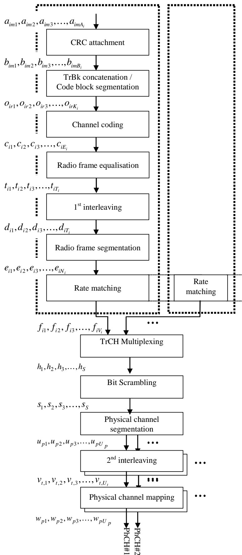
Figure 1: Transport channel multiplexing structure for uplink and downlink for 3.84Mcps and 7.68 Mcps TDD
