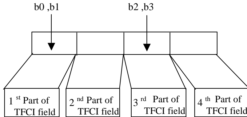
Figure 10: Mapping of TFCI code word bits to TFCI position in 1.28 Mcps TDD option, when N_{\text{TFCI code word}}=4
