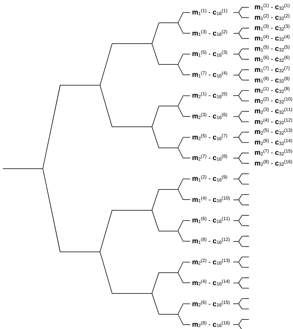
Figure 18AK: Association of midambles to channelisation codes for PRACH in the OVSF tree
