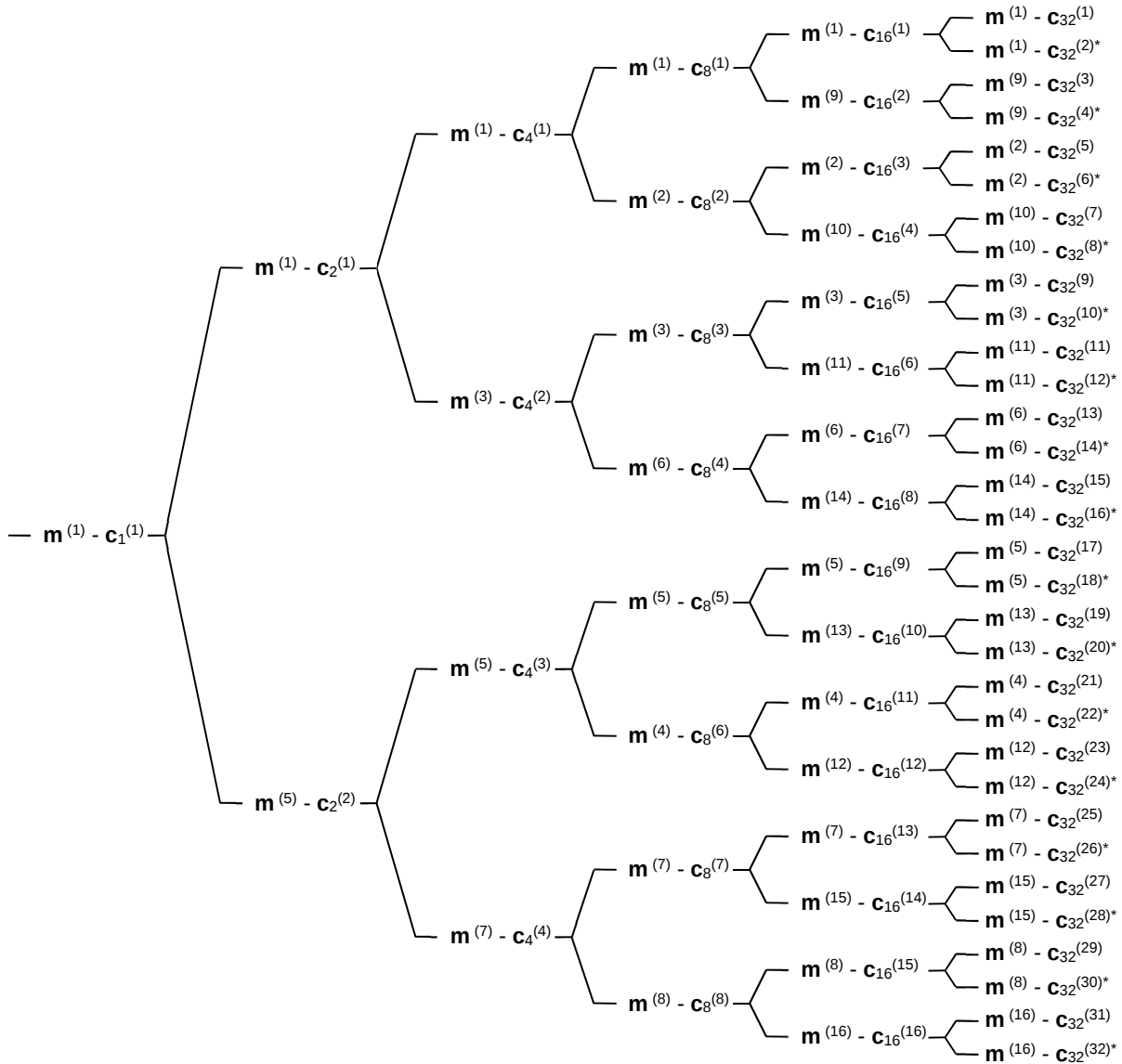
Figure AB.1: Association of Midambles to Spreading Codes for K_{\text{Cell}} = 16
