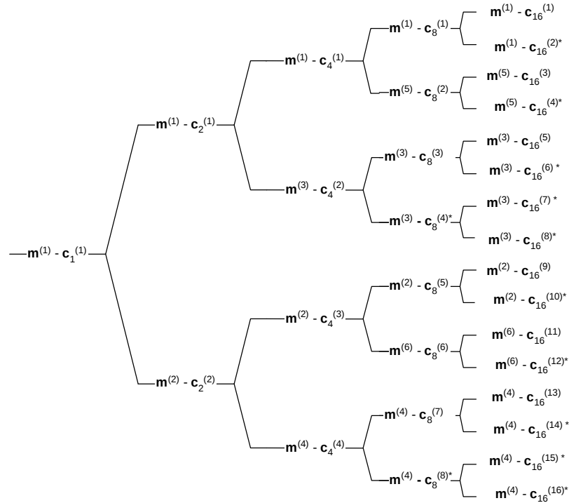
Figure A.4: Association of Midambles to Spreading Codes for Burst Type 2 and K_{\text{Cell}}=6
