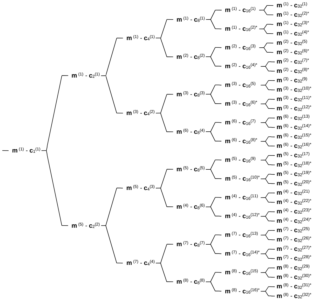
Figure AB.2: Association of Midambles to Spreading Codes for K_{\text{Cell}} = 8
