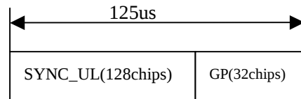
Figure 18J: burst structure of the UpPCH (UpPTS)
