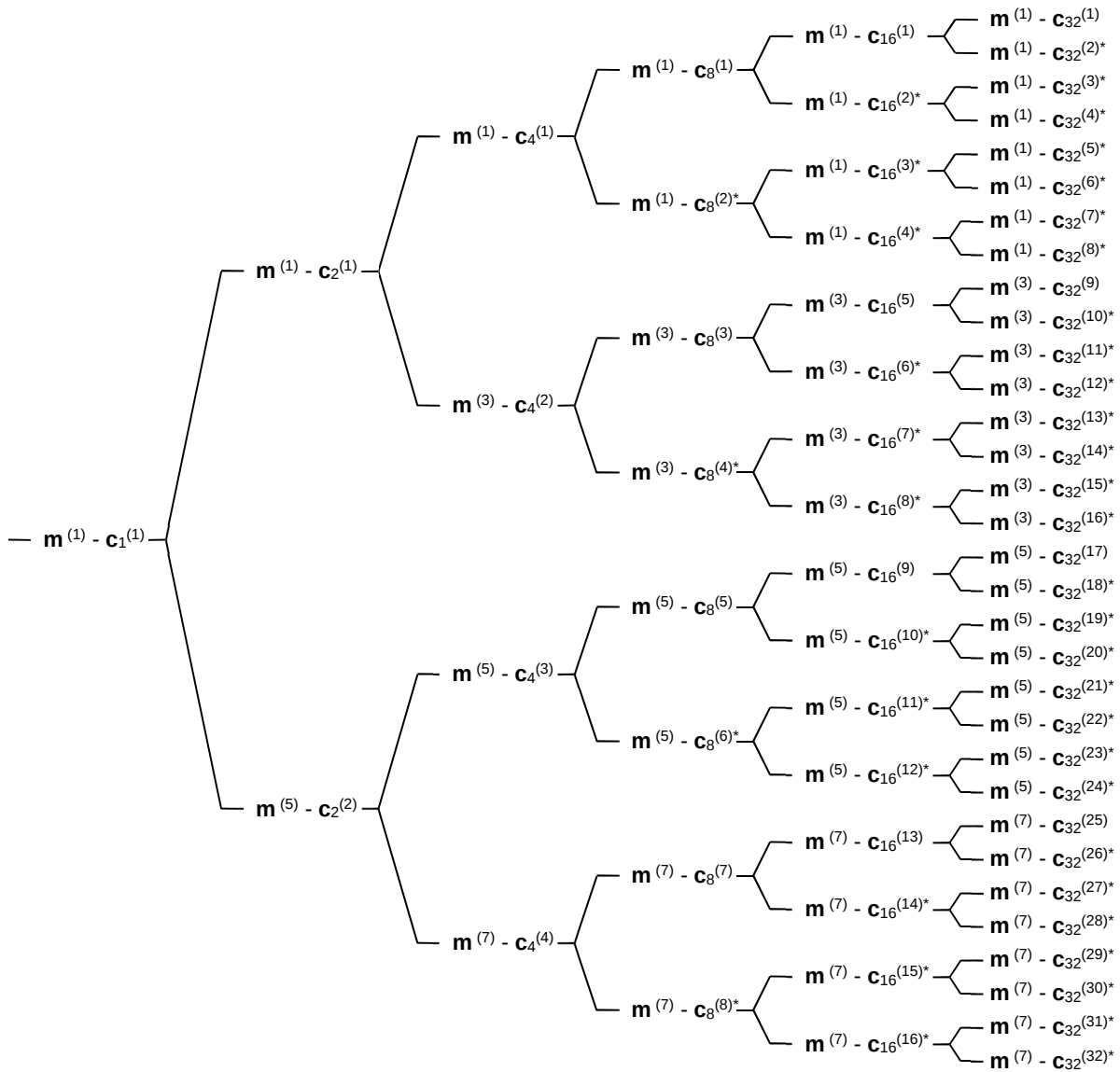
Figure AB.3: Association of Midambles to Spreading Codes for K_{\text{Cell}} = 4
