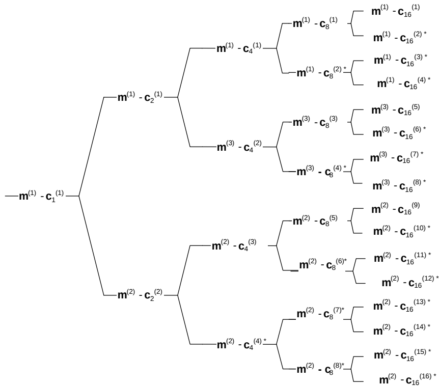
Figure A.5: Association of Midambles to Spreading Codes for Burst Type 2 and K_{\text{Cell}}=3
