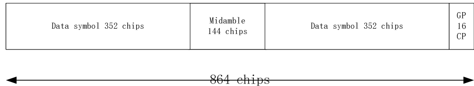
Figure 18P: E-PUCH data burst without E-UCCH/TPC
