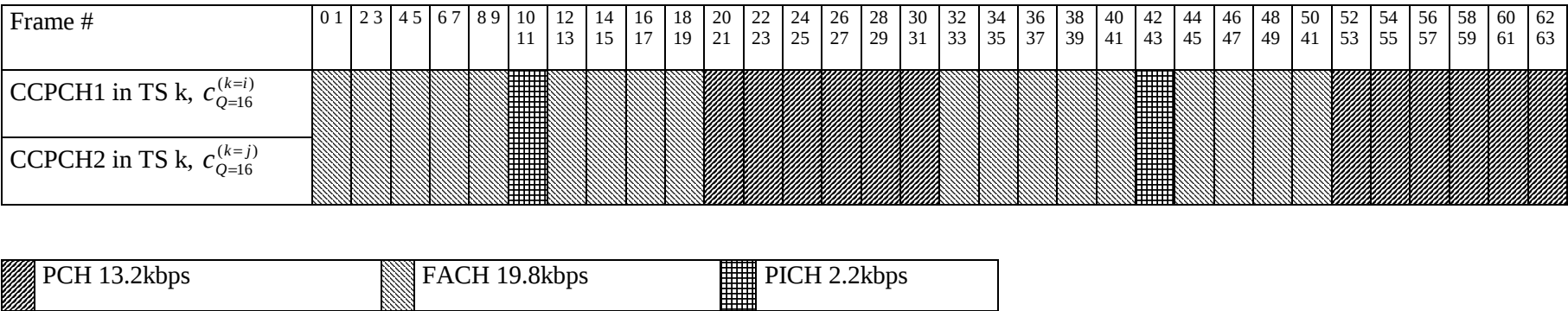
Figure CA.2: Example for a multiframe structure for S-CCPCHs and PICH that is repeated every 64th frame, i,j=1...16 (i≠j), k≠0, 1, (128 sub-frame)
