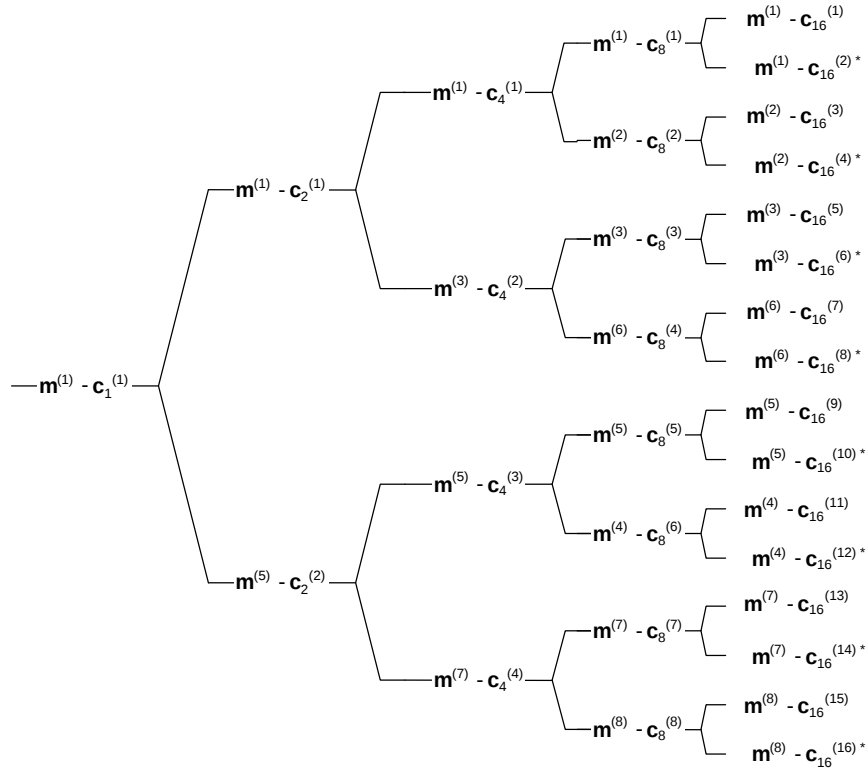
Figure A.2: Association of Midambles to Spreading Codes for Burst Type 1/3 and K_{\text{Cell}}=8
