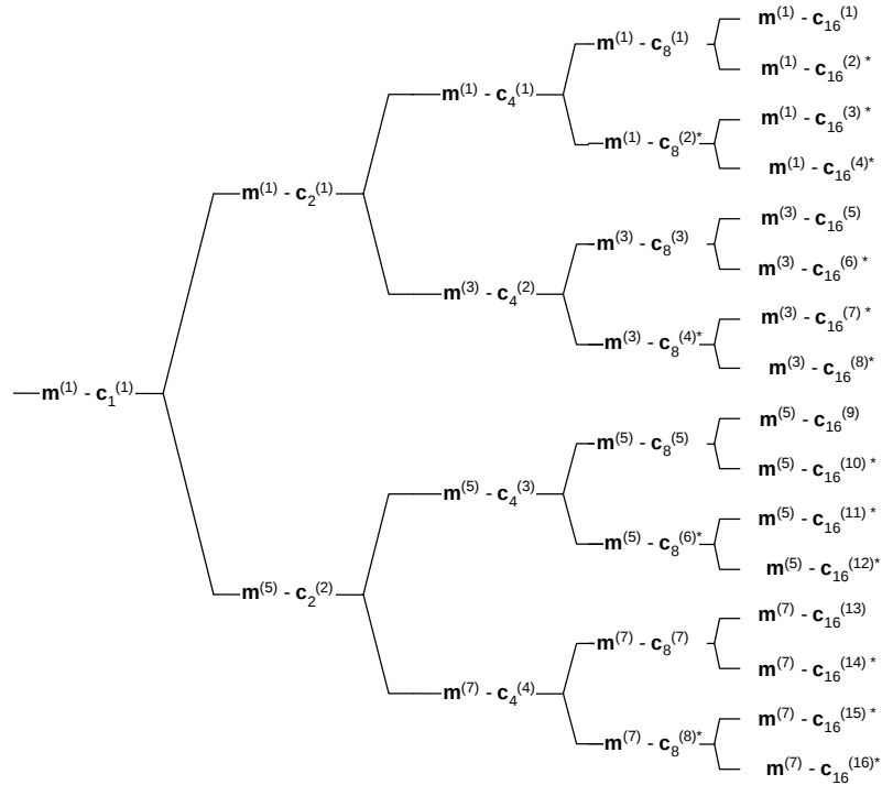
Figure A.3: Association of Midambles to Spreading Codes for Burst Type 1/3 and K_{\text{Cell}}=4
