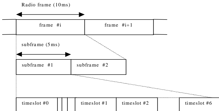
Figure 19: Physical channel signal format for 1.28Mcps TDD option
