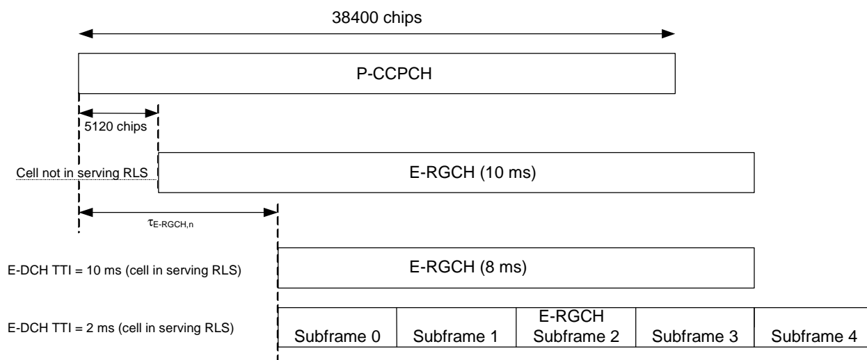
Figure 38: E-RGCH timing
