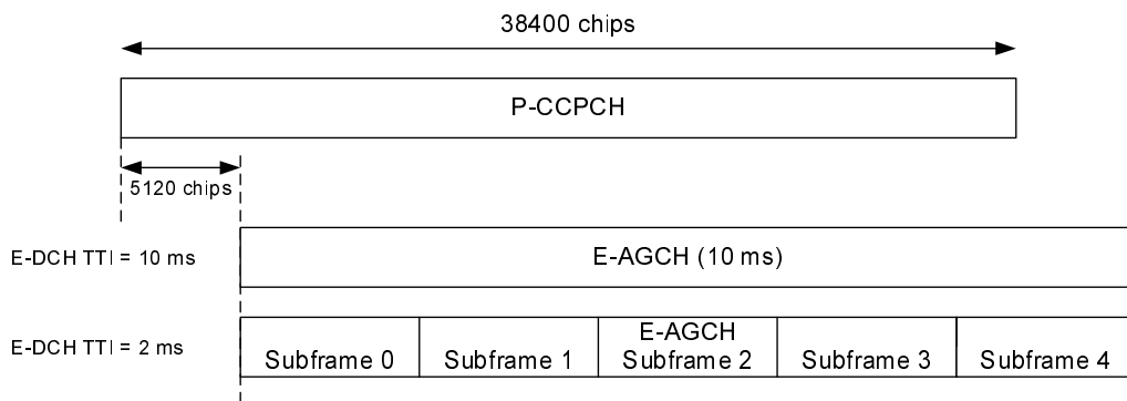
Figure 39: E-AGCH timing
