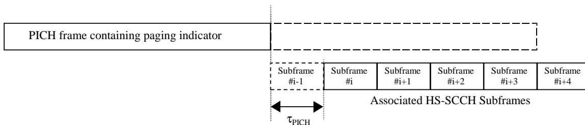
Figure 30a: Timing relation between PICH frame and associated HS-SCCH subframes
