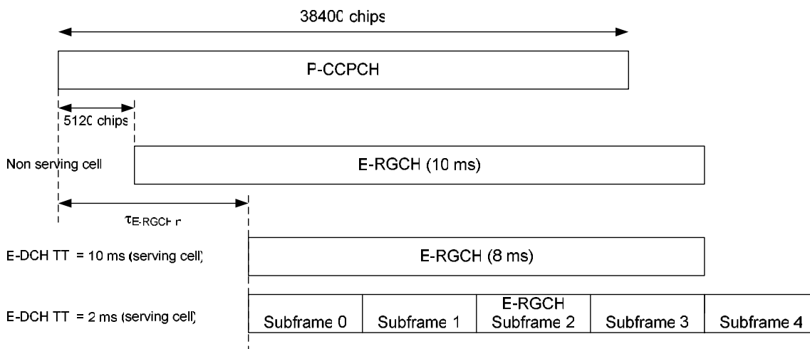
Figure 38: E-RGCH timing
