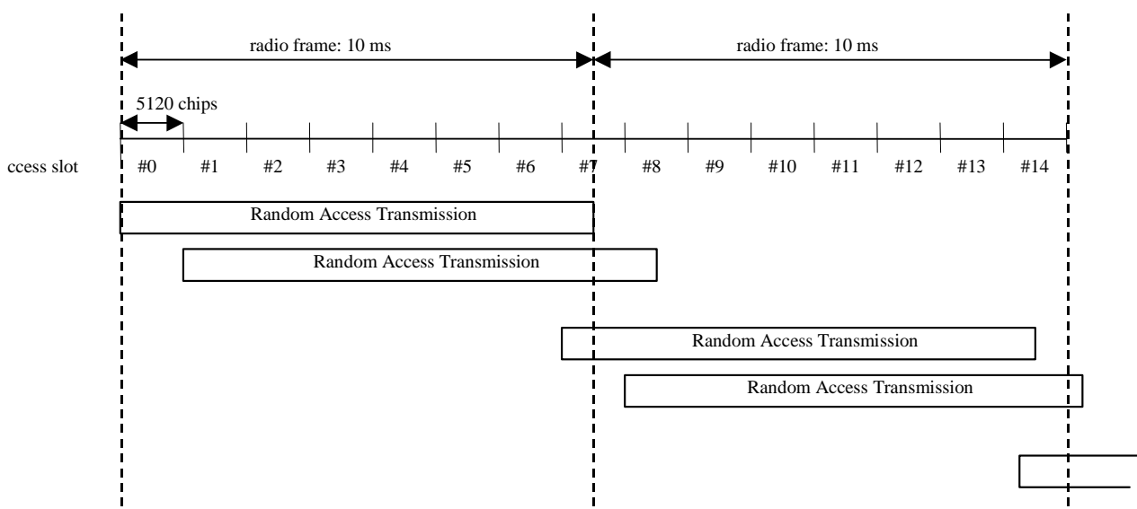
Figure 4: RACH access slot numbers and their spacing
