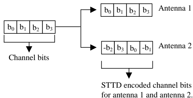
Figure 9: Generic block diagram of the STTD encoder
