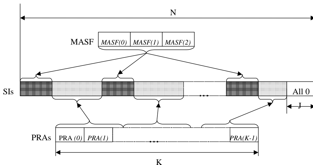
Figure 27: Mapping of MASF and PRAs to SIs in CSICH
