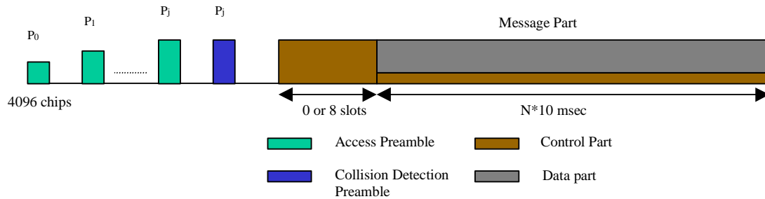
Figure 7: Structure of the CPCH access transmission
