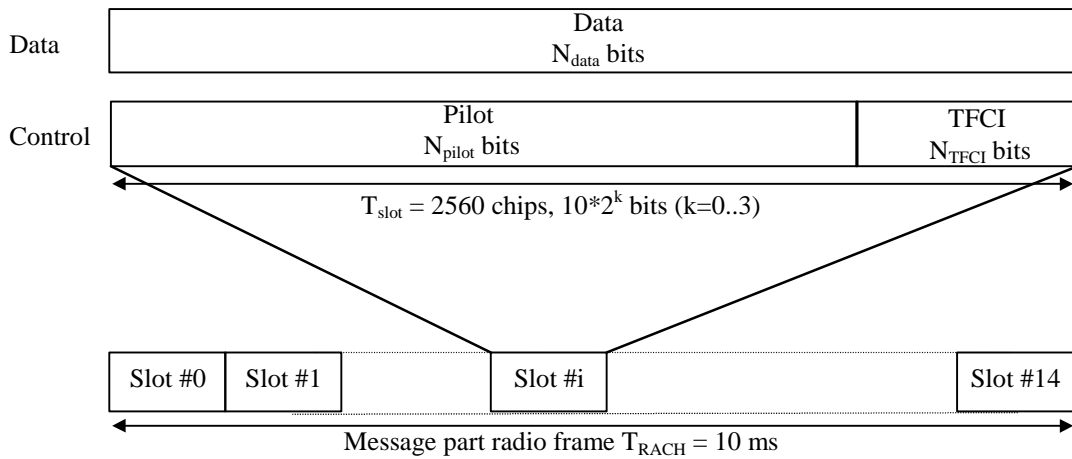
Figure 6: Structure of the random-access message part radio frame
