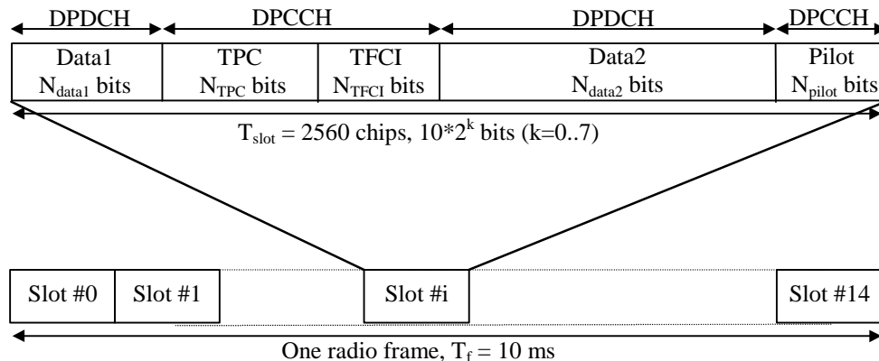
Figure 10: Frame structure for downlink DPCH
