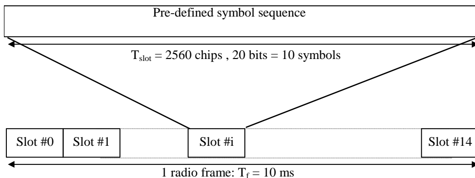
Figure 14: Frame structure for Common Pilot Channel
