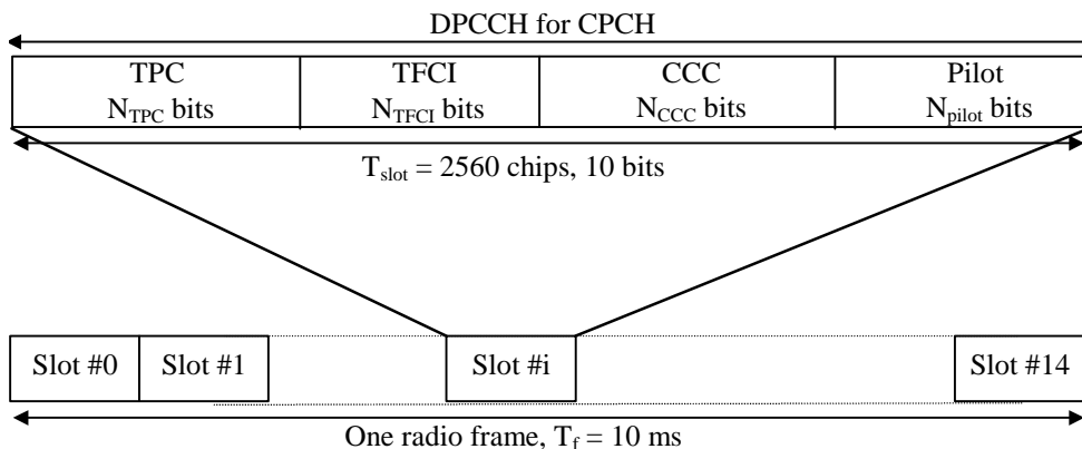
Figure 13: Frame structure for downlink DPCCH for CPCH
