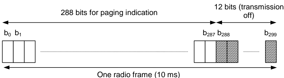
Figure 25: Structure of Paging Indicator Channel (PICH)
