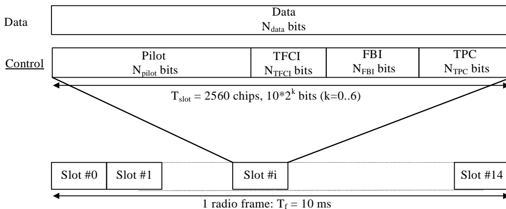
Figure 8: Frame structure for uplink Data and Control Parts Associated with PCPCH
