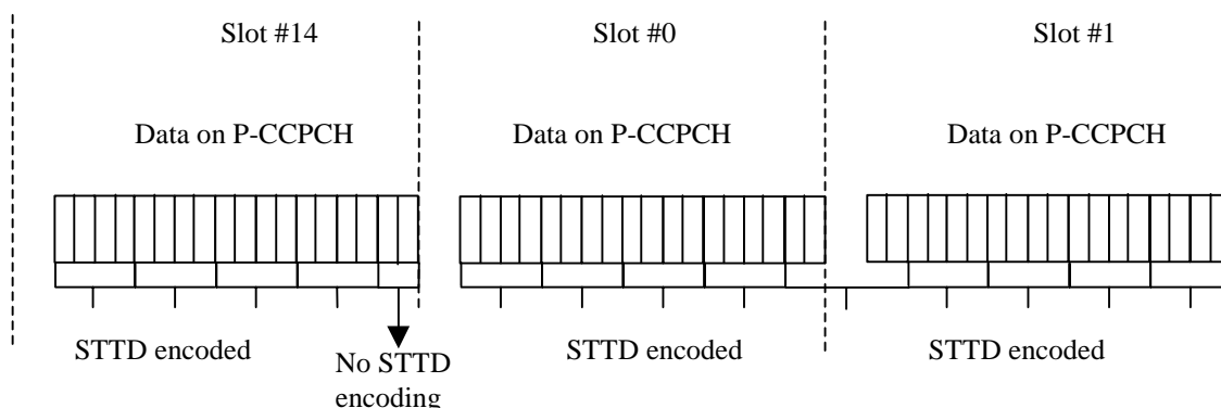
Figure 17: STTD encoding for the data bits of the P-CCPCH
