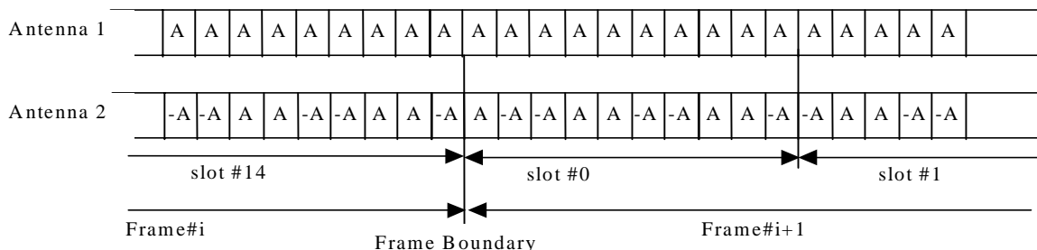
Figure 15: Modulation pattern for Common Pilot Channel (with A = 1+j )
