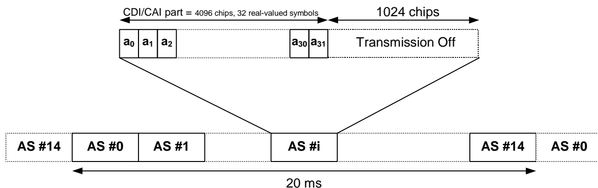
Figure 24: Structure of CD/CA Indicator Channel (CD/CA-ICH)
