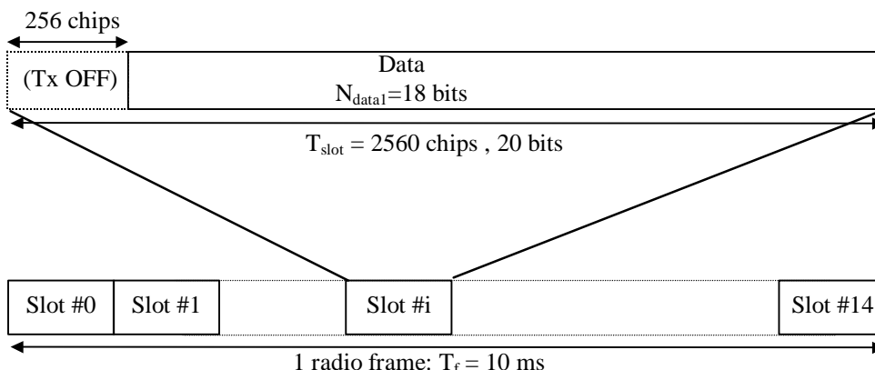
Figure 16: Frame structure for Primary Common Control Physical Channel
