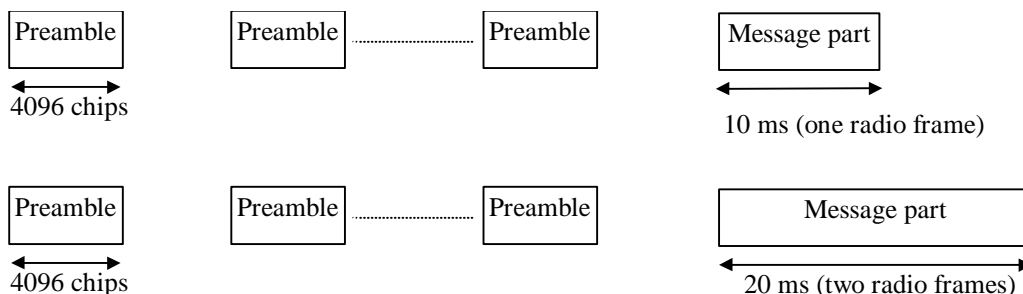
Figure 5: Structure of the random-access transmission
