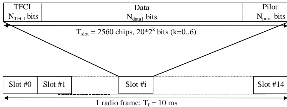
Figure 18: Frame structure for Secondary Common Control Physical Channel
