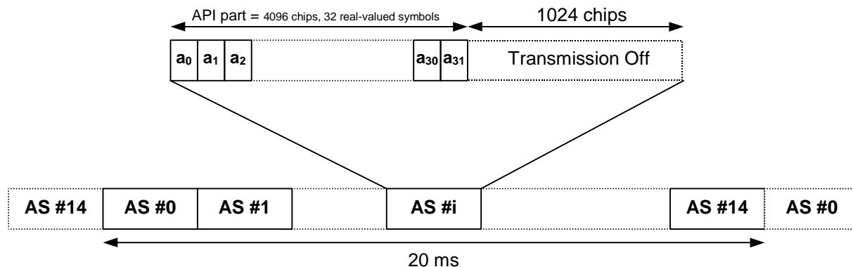
Figure 23: Structure of AP Acquisition Indicator Channel (AP-AICH)
