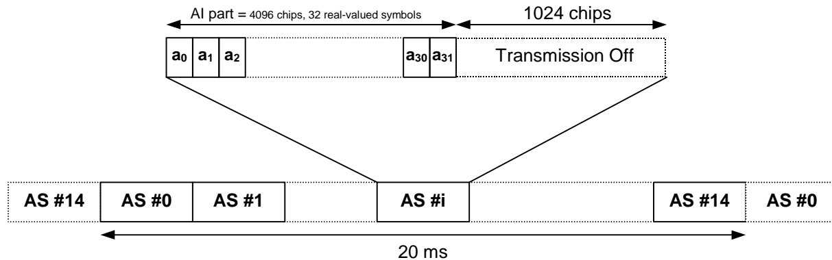
Figure 22: Structure of Acquisition Indicator Channel (AICH)
