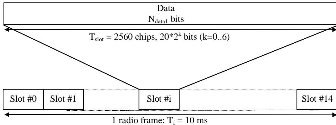
Figure 21: Frame structure for the PDSCH
