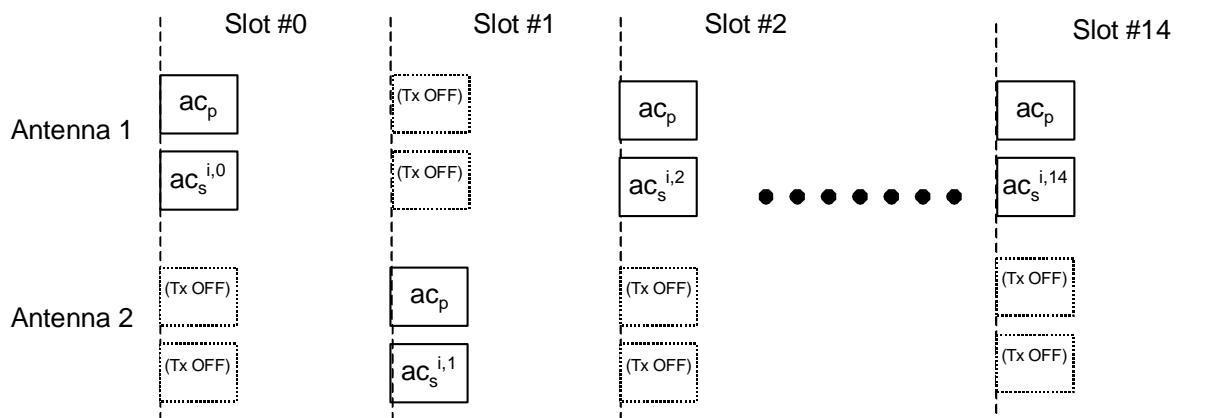
Figure 20: Structure of SCH transmitted by TSTD scheme
