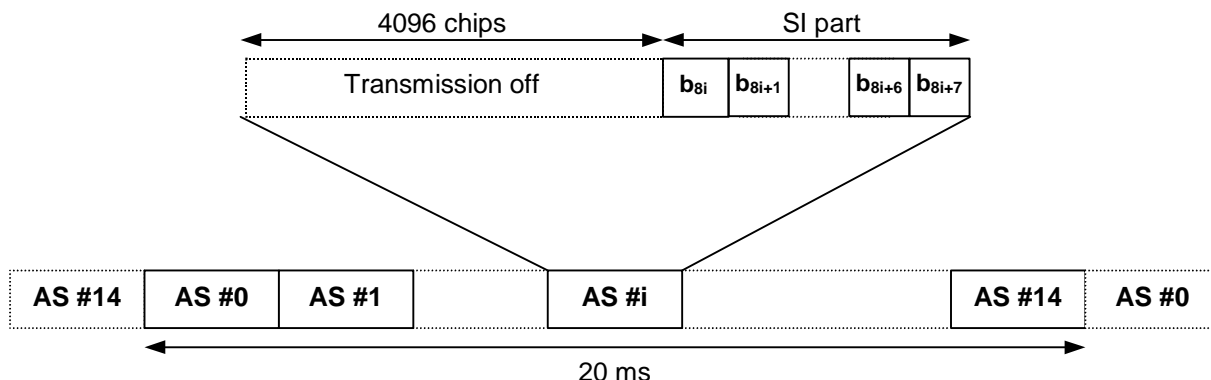
Figure 26: Structure of CPCH Status Indicator Channel (CSICH)
