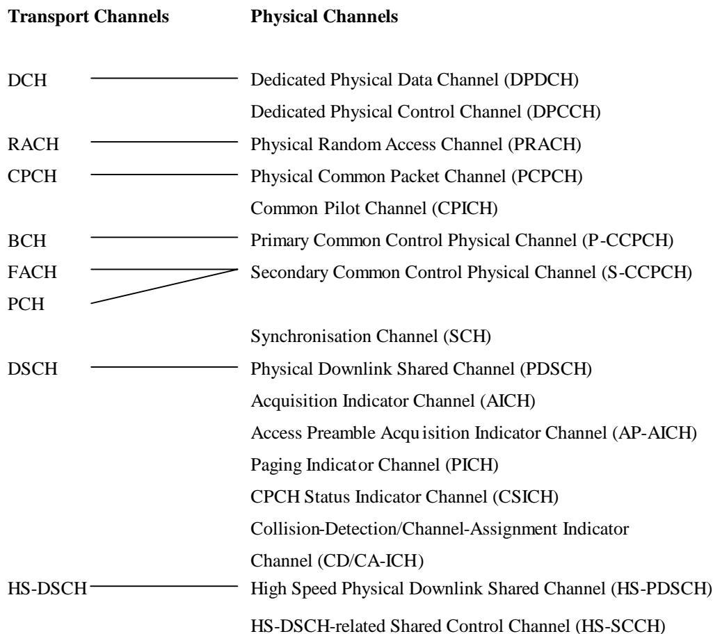
Figure 30: Transport-channel to physical-channel mapping
