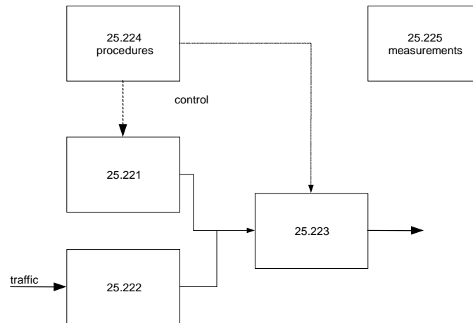
Figure 3 - TDD layer 1 functions relationships by specification
