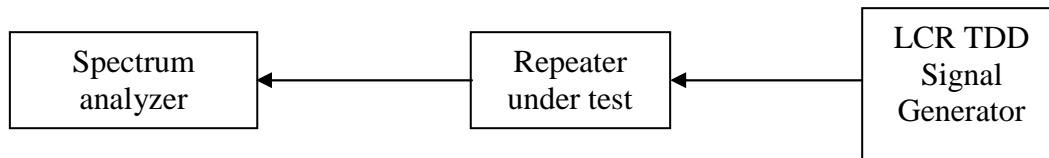
Figure A.7: Measuring system set-up for modulation accuracy: peak code domain error.
