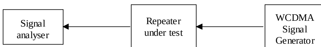
Figure A.7: Measuring system set-up for modulation accuracy: peak code domain error and relative coder domain error.
