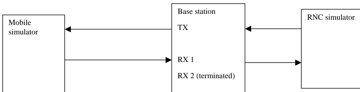
Figure 1: Communication link set up for BS immunity measurement
