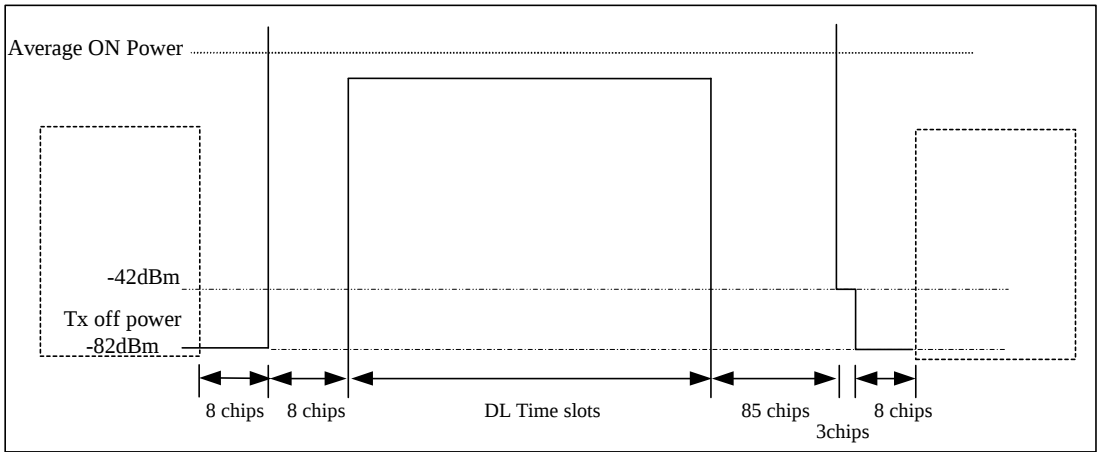
Figure 6.1A: Transmit ON/OFF template
