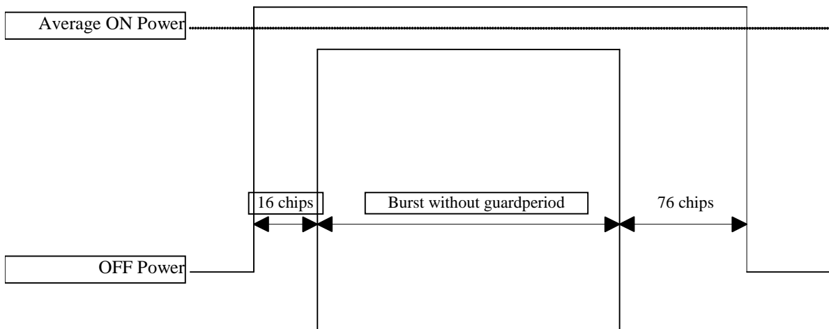
Figure 6.1: Transmit ON/OFF template
