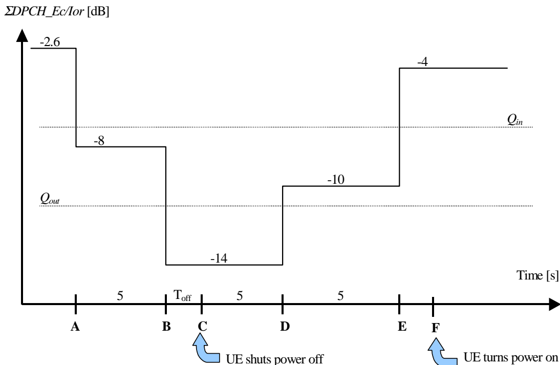
Figure 6.1AA: Conditions for out-of-synch handling in the UE. The indicated thresholds Q_{out} and Q_{in} are only informative.
