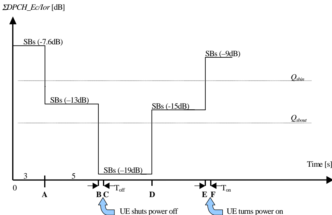
Figure 6.1A. Conditions for out-of-synch handling in the UE - discontinuous transmission. The indicated thresholds Q_{s\text{bout}} and Q_{s\text{bin}} are only informative.
