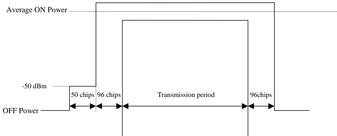
Figure 6.2: Transmit ON/OFF template
