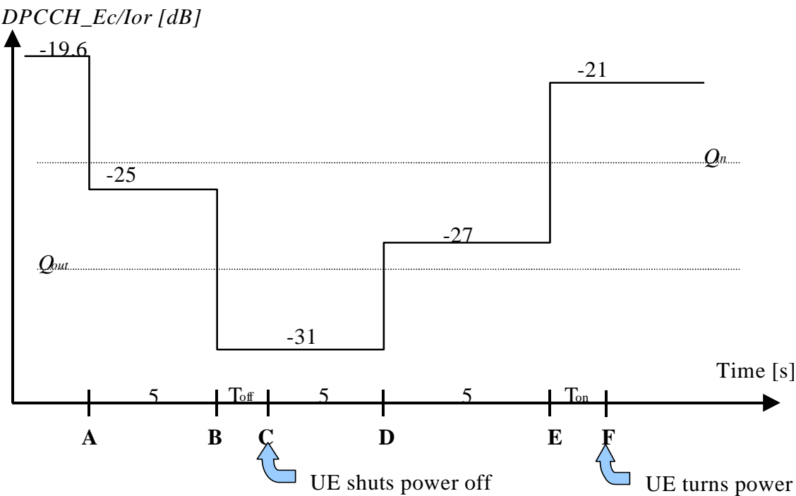
Figure 6.1A: Test case for out-of-synch handling in the UE supporting the enhanced performance requirements type1
