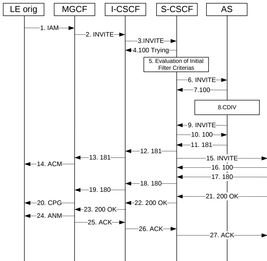
Figure A.6b: Call Forwarding Unconditional
