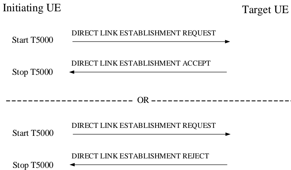
Figure 6.1.2.2.2: UE oriented PC5 unicast link establishment procedure
