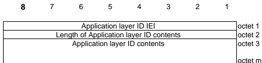
Figure 8.4.4.1: Application layer ID information element
