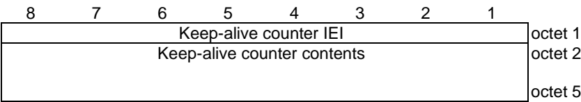
Figure 8.4.10.1: Keep-alive counter information element
