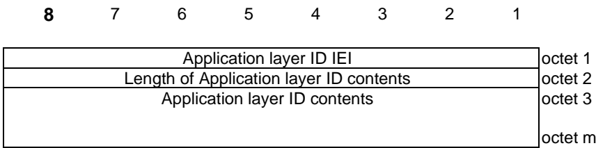
Figure 8.4.4.1: Application layer ID information element
