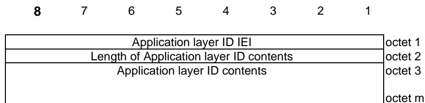
Figure 8.4.4.1: Application layer ID information element
