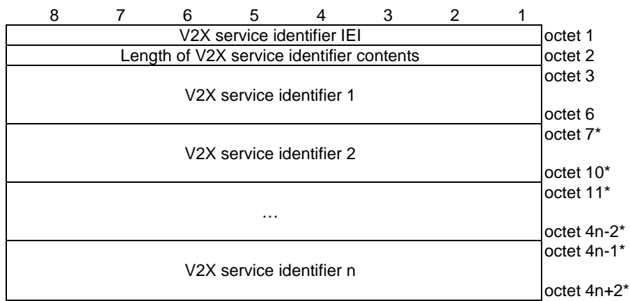
Figure 8.4.3.1: V2X service identifier information element
