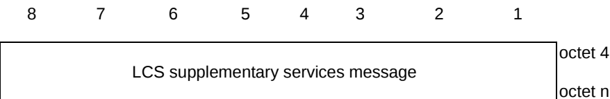
Figure 11.2.1.3: LCS-UP payload contents with LCS-UP payload type "LCS supplementary services message"
