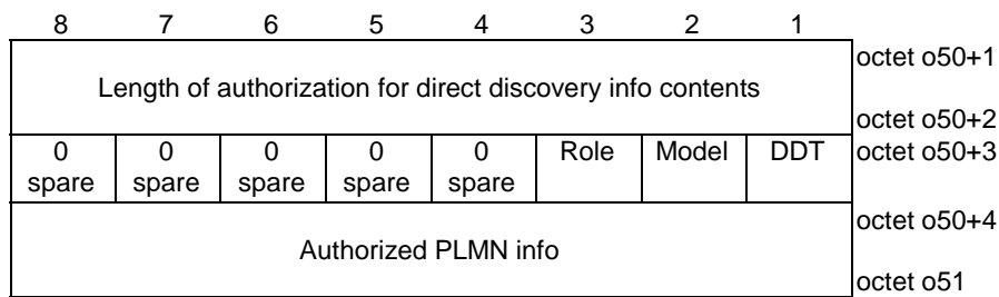
Figure 5.3.2.3: Authorization for direct discovery info
