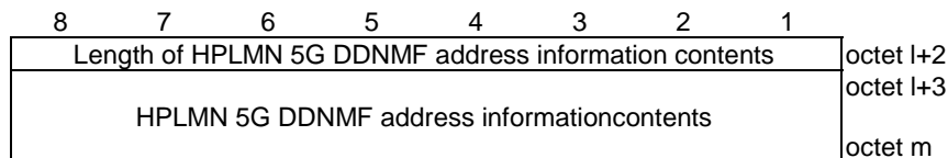
Figure 5.3.2.17: HPLMN 5G DDNMF address information
