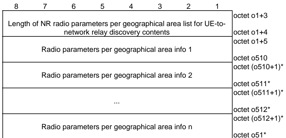
Figure 5.6.2.6: NR radio parameters per geographical area list for UE-to-network relay discovery
