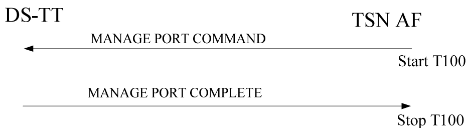
Figure 5.2.1.2.1: Network-requested port management procedure
