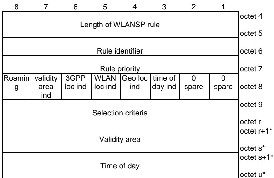
Figure 5.3.2.3: WLANSP rule
