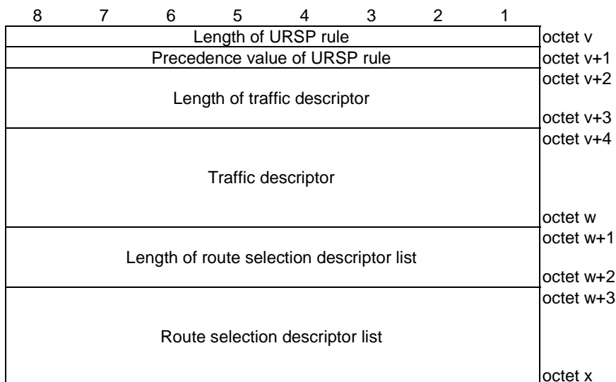
Figure 5.2.2: URSP rule
