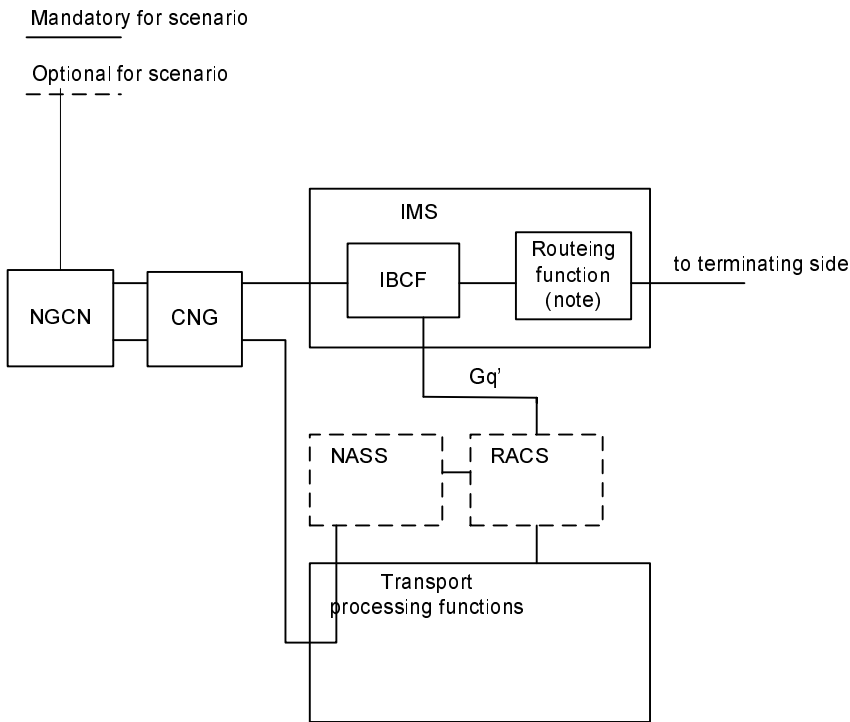
NOTE: One or more routeing functions can appear in the originating side for this scenario. Figure 7.1.1: Session level virtual leased line scenario originating functional entities
