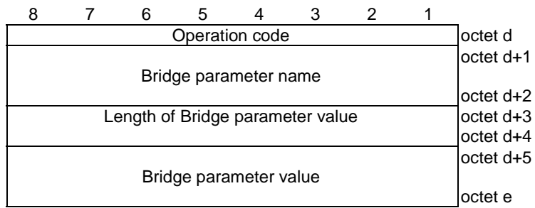
Figure 9.5B.5: Operation for operation code set to "0000011" and "0001001"
