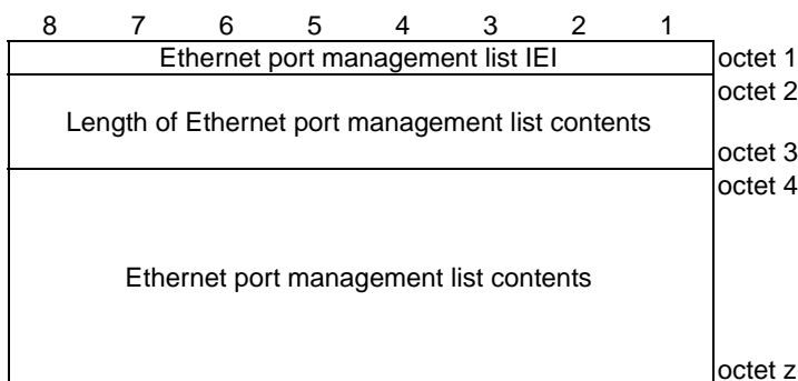
Figure 9.2.1: Ethernet port management list information element
