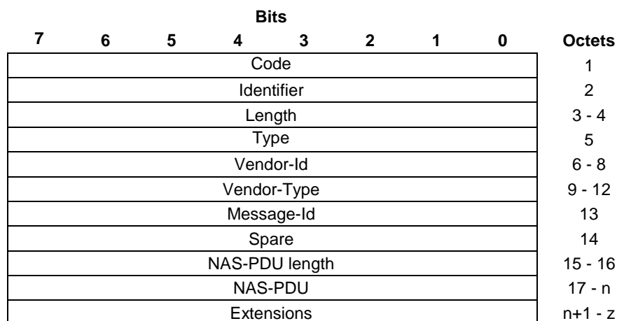
Figure 9.3.2.2.3-1: EAP-Request/5G-NAS message
