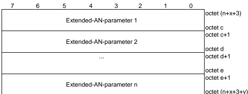
Figure 9.3.2.2-4: Extended-AN-parameters field
