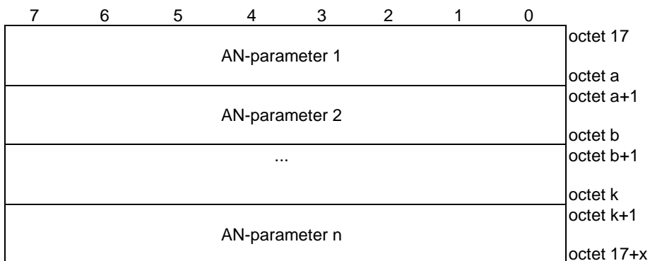
Figure 9.3.2.2.2-2: AN-parameters field
