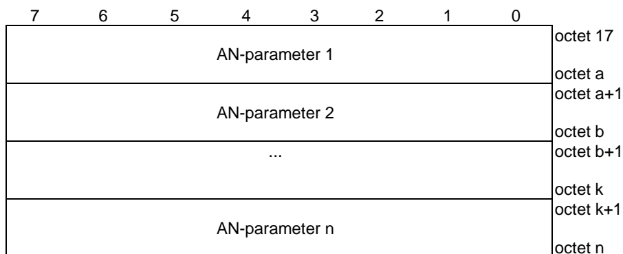
Figure 9.3.2.2.5-2: AN-parameters field
