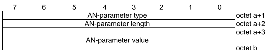
Figure 9.3.2.2.5-3: AN-parameter field
