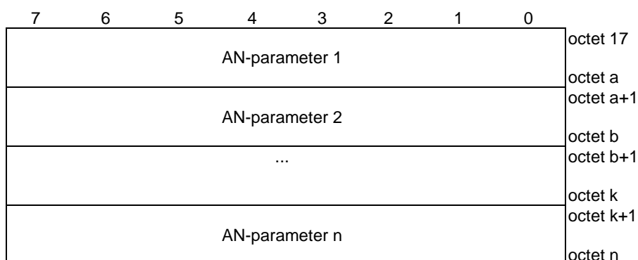
Figure 9.3.2.2.5-2: AN-parameters field
