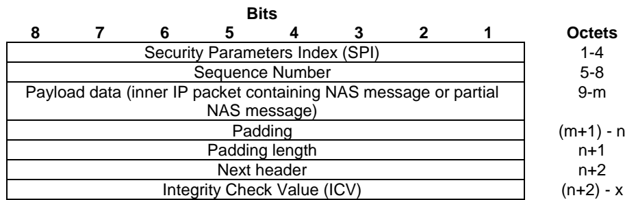
Figure 8.2.2-1: ESP packet format
