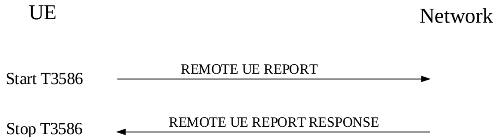
Figure 6.6.2.2.1: Remote UE report procedure
