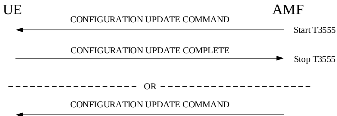
Figure 5.4.4.1.1: Generic UE configuration update procedure
