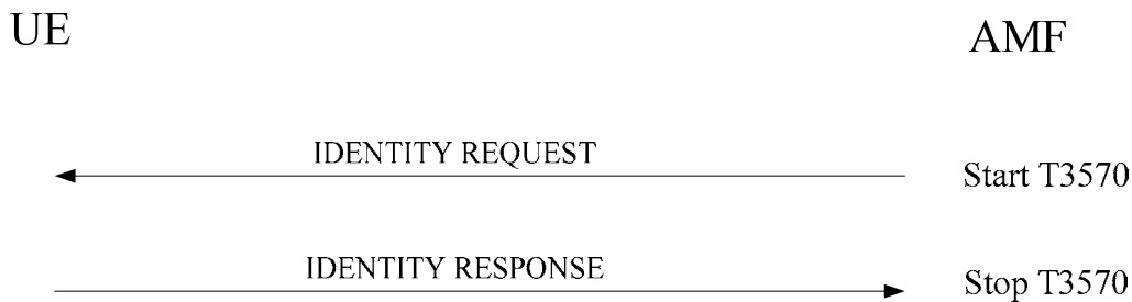
Figure 5.4.3.2.1: Identification procedure
