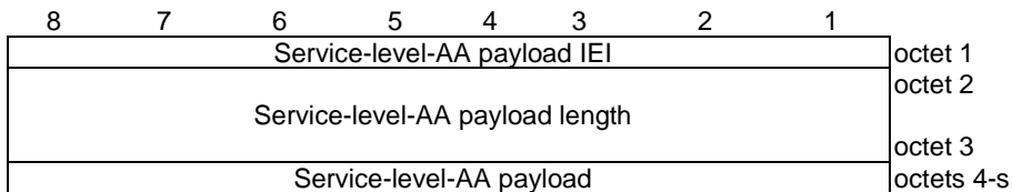
Figure 9.11.2.13.1: Service-level-AA payload information element
