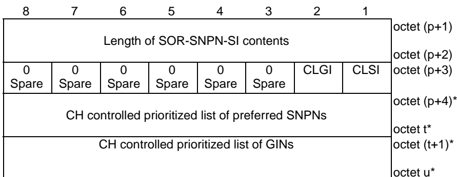
Figure 9.11.3.51.9: SOR-SNPN-SI
