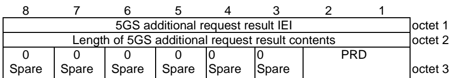
Figure 9.11.3.81.1: 5GS additional request result information element
