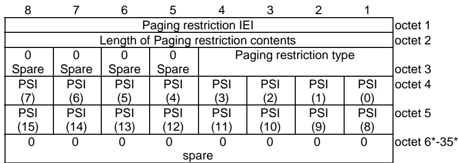
Figure 9.11.3.77.2: Paging restriction information element for Paging restriction type = "All paging is restricted except for specified PDU session(s)" and for Paging restriction type = "All paging is restricted except for voice service and specified PDU session(s)"
