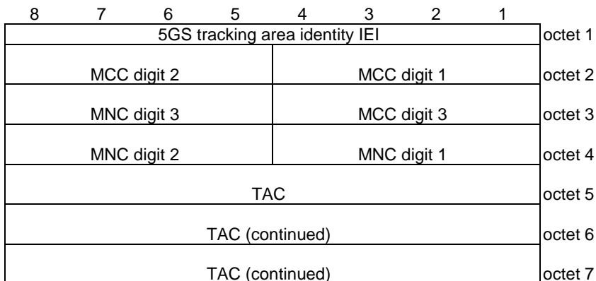
Figure 9.11.3.8.1: 5GS tracking area identity information element
