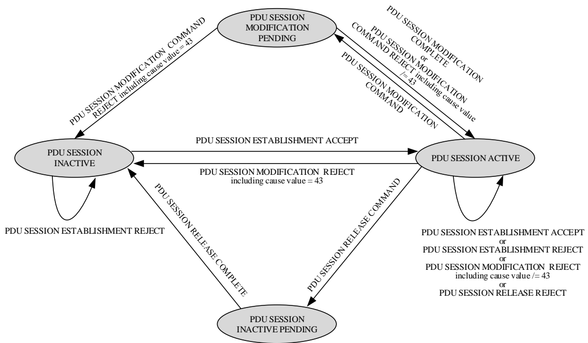
Figure 6.1.3.3.1: The 5GSM sublayer states for PDU session handling in the network (overview)
