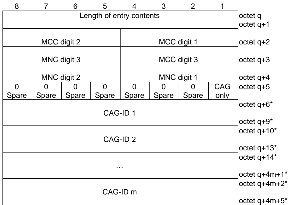
Figure 9.11.3.86.2: Entry n
