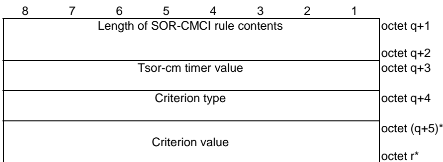
Figure 9.11.3.51.8: SOR-CMCI rule
