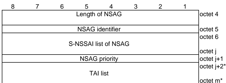
Figure 9.11.3.87.2: NSAG
