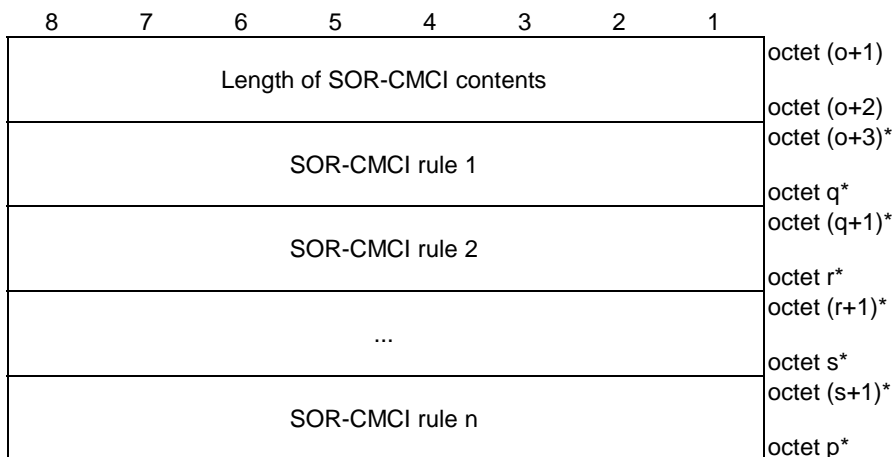
Figure 9.11.3.51.7: SOR-CMCI
