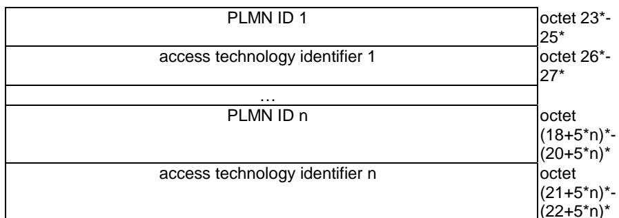
Figure 9.11.3.51.3: PLMN ID and access technology list (m=22+5*n)
