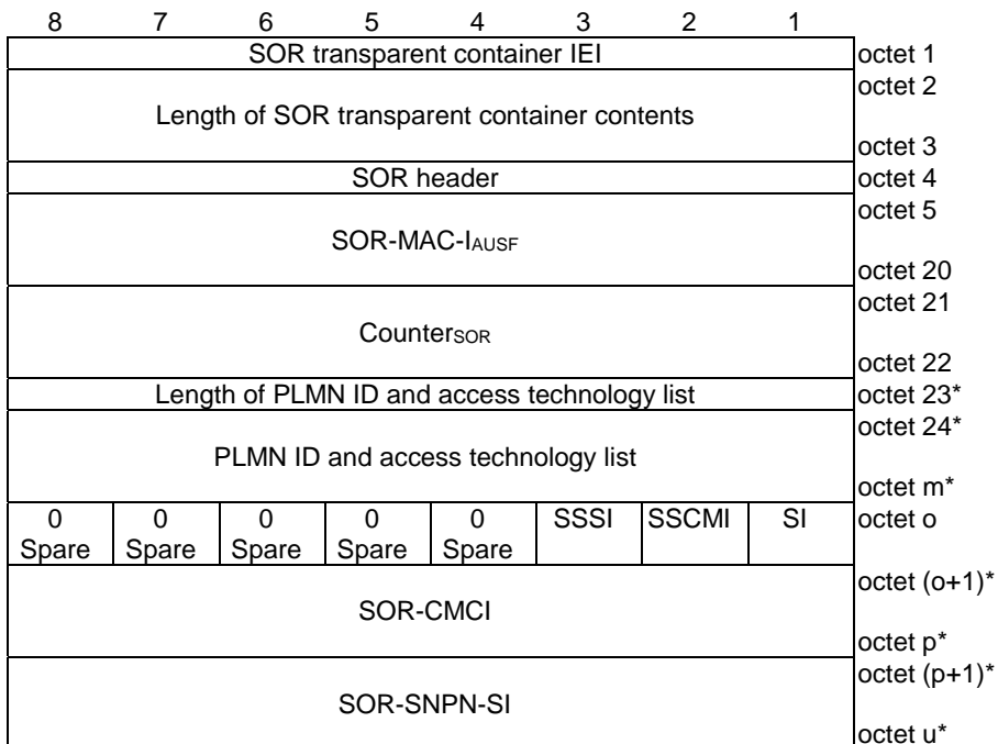
Figure 9.11.3.51.2A: SOR transparent container information element for list type with value "1", SOR data type with value "0", additional parameters with value "1"
