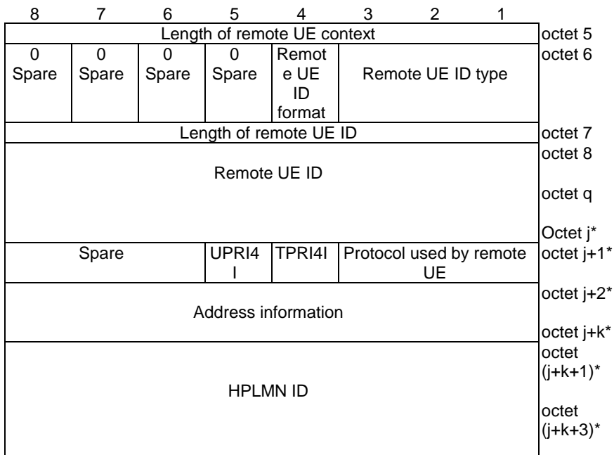
Figure 9.11.4.29.2: Remote UE context
