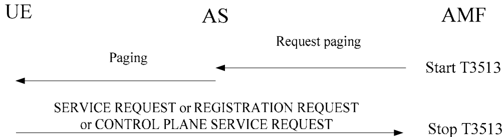
Figure 5.6.2.2.1.1: Paging procedure
