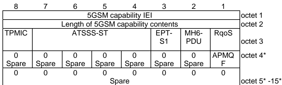
Figure 9.11.4.1.1: 5GSM capability information element
