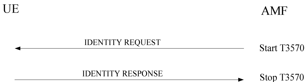
Figure 5.4.3.2.1: Identification procedure
