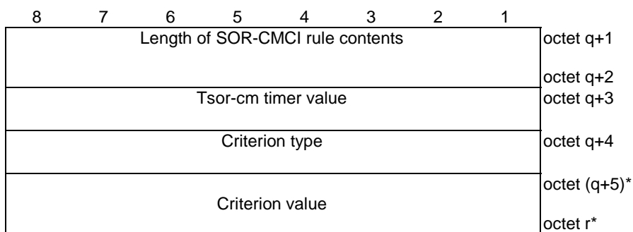
Figure 9.11.3.51.8: SOR-CMCI rule
