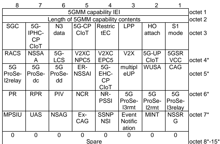
Figure 9.11.3.1.1: 5GMM capability information element
