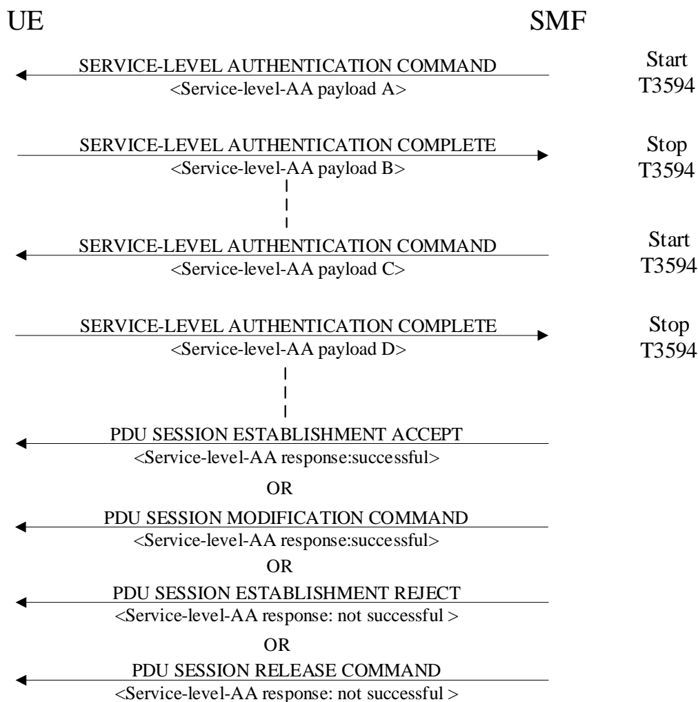
Figure 6.3.1A.1-1: Service-level authentication and authorization procedure
