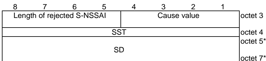
Figure 9.11.3.46.2: Rejected S-NSSAI
