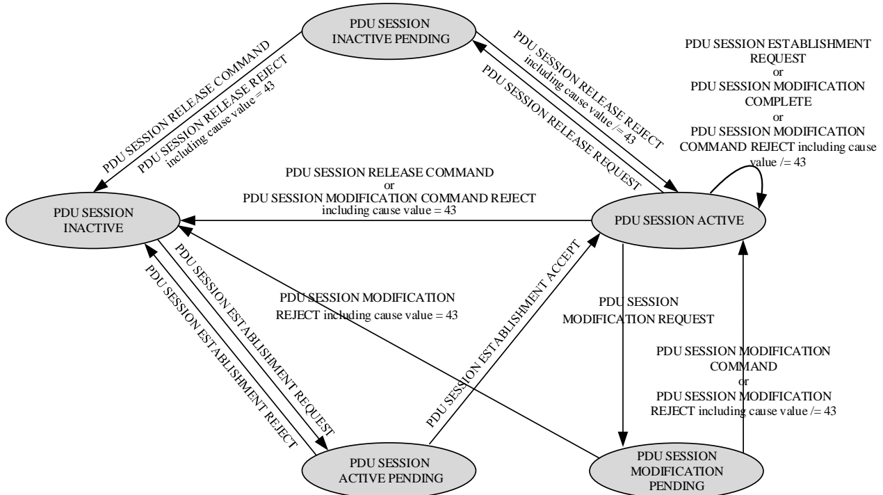
Figure 6.1.3.2.1.1: The 5GSM sublayer states for PDU session handling in the UE (overview)
