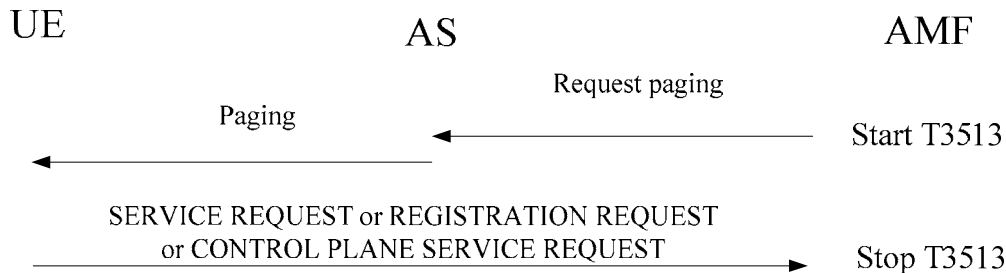
Figure 5.6.2.2.1.1: Paging procedure
