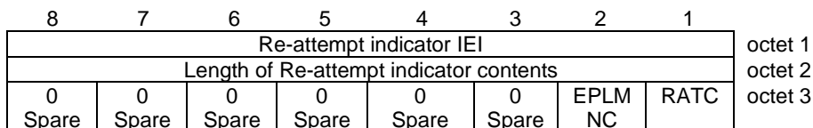
Figure 9.11.4.17.1: Re-attempt indicator
