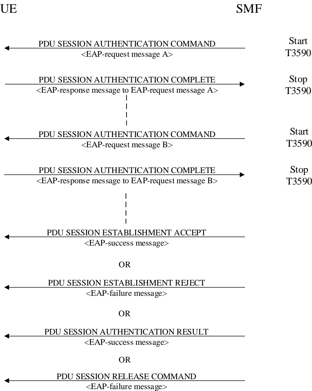
Figure 6.3.1.1: PDU session authentication and authorization procedure
