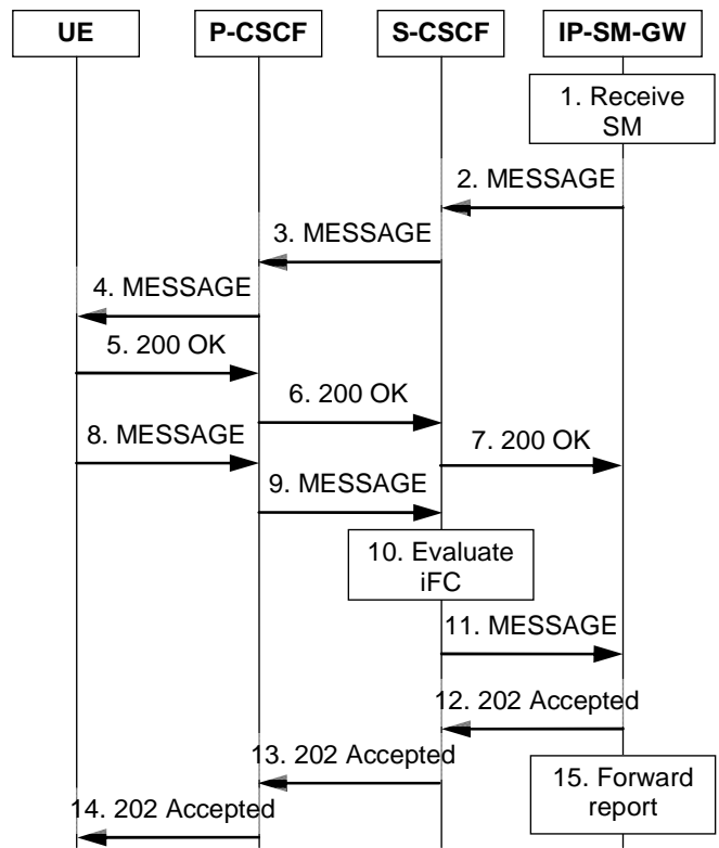
Figure B.6-1: UE originated SM deliver procedure over IP signalling
