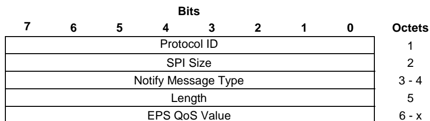
Figure 8.2.9.10-1: EPS_QOS Notify payload format
