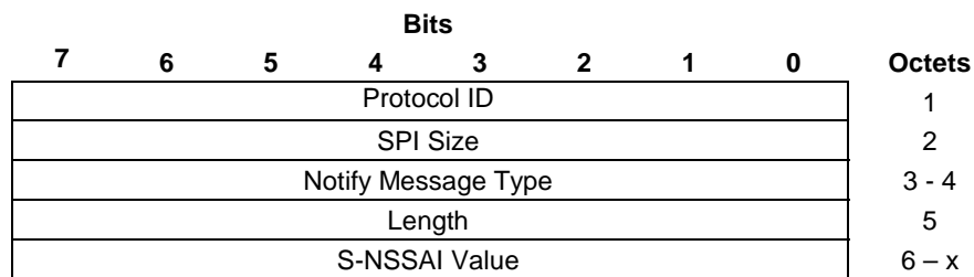
Figure 8.2.9.16-1: N1_MODE_INFORMATION Notify payload format
