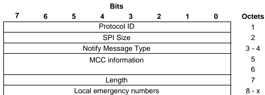
Figure 8.2.9.8-1: EMERGENCY_CALL_NUMBERS Notify payload
