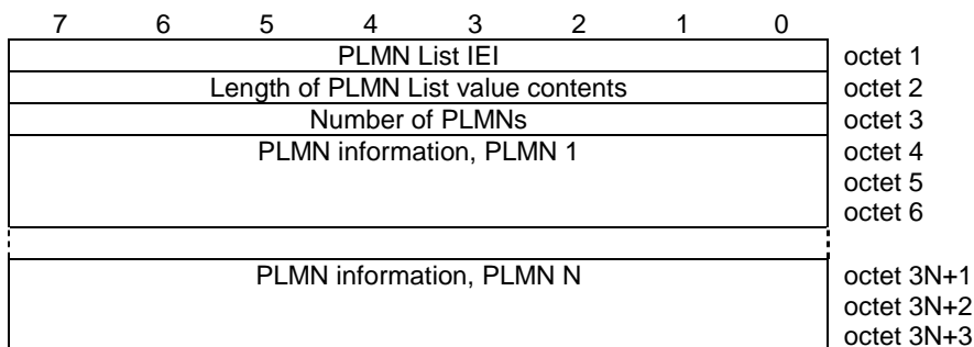
Figure H.2.4.2-1: PLMN List information element
