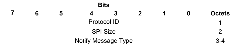
Figure 8.2.9.4-1: P-CSCF_RESELECTION_SUPPORT Notify Payload format
