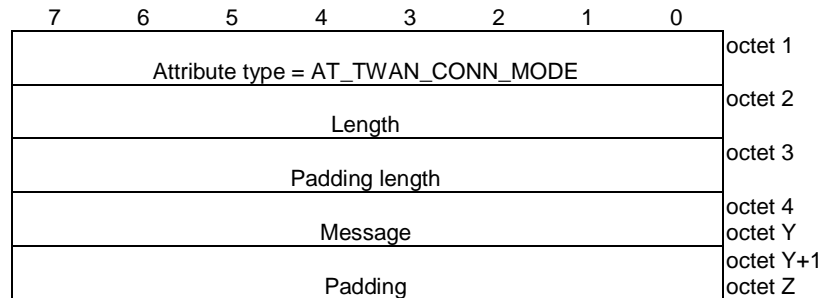
Figure 8.2.7.1-1: AT_TWAN_CONN_MODE attribute
