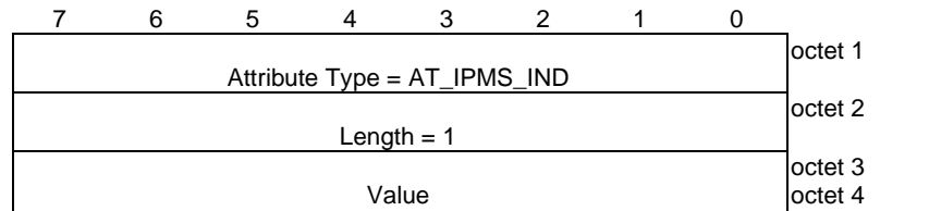
Figure 8.2.1.1: AT_IPMS_IND attribute
