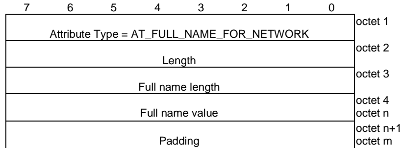
Figure 8.2.5.1-1: AT_FULL_NAME_FOR_NETWORK attribute
