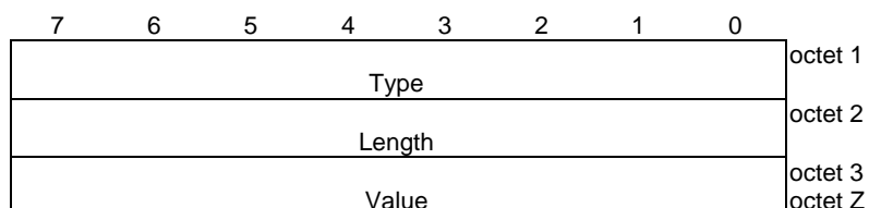
Figure 8.1.4.2-1: Item
