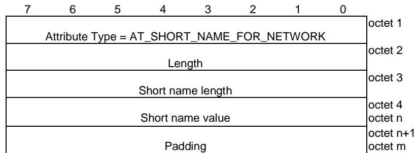
Figure 8.2.5.2-1: AT_SHORT_NAME_FOR_NETWORK attribute
