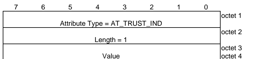
Figure 8.2.3.1-1: AT_TRUST_IND attribute
