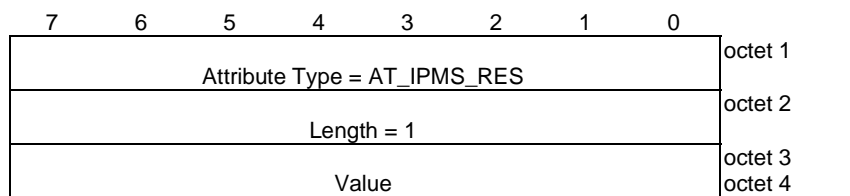
Figure 8.2.1.2: AT_IPMS_RES attribute.
